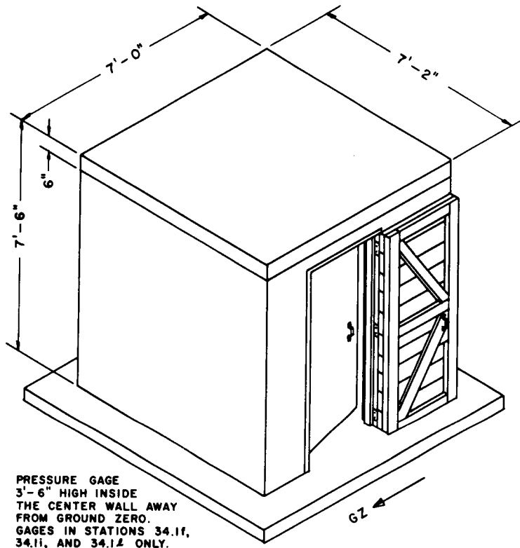
Fig. 14—Sketch of utility-type shelter, stations 1-34.1 e to m.
